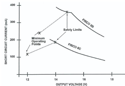
Permitted Safety Description For FISCO Power Supply
