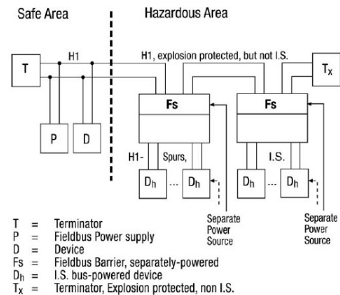
Figure 12: Separate powered Fieldbus Barrier
